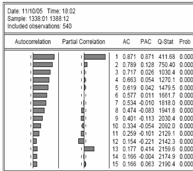
Correlogram of MOVRWPI
