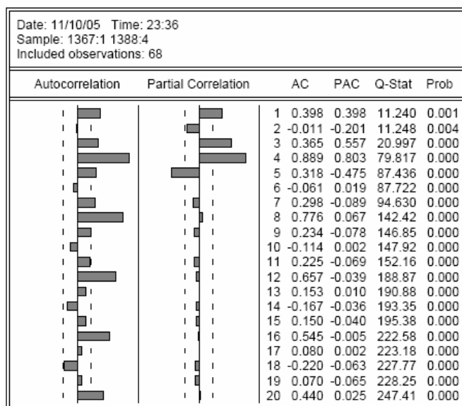
Correlogram of LAV
