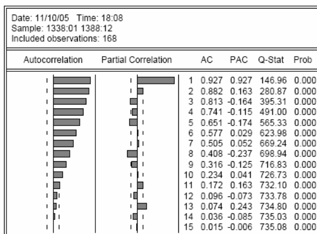
Correlogram of MOVRPPI
